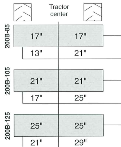
Rotavator 200-105. Specially designed for compact tractors.
